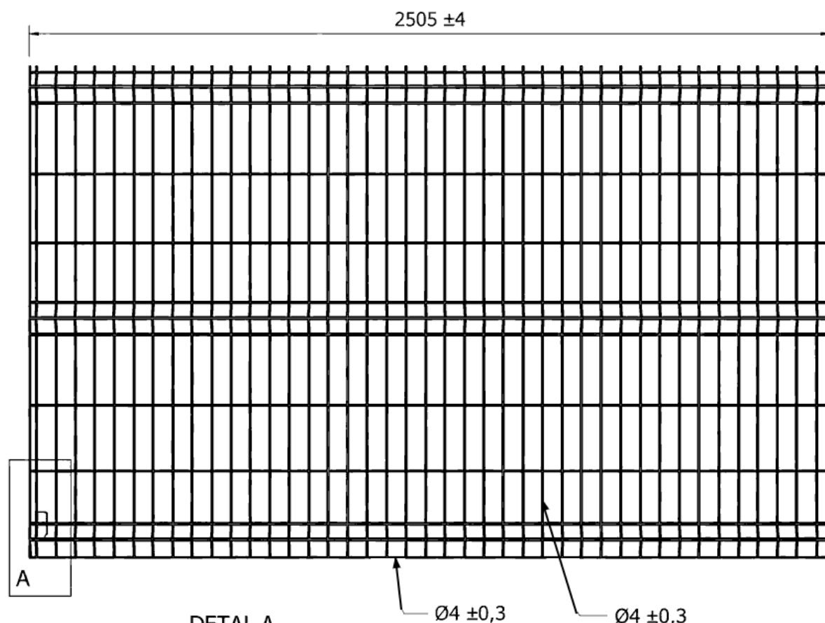
DETAL A (1:5)
