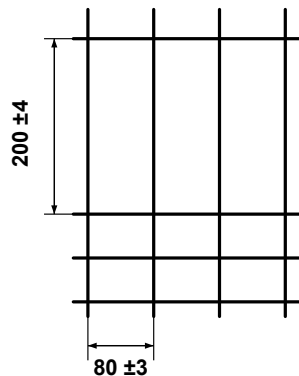
DETAL A (1:5)
