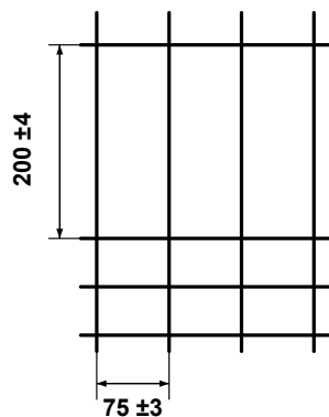
DETAL A (1:5)
