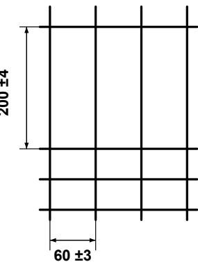
DETAL A (1:5)
